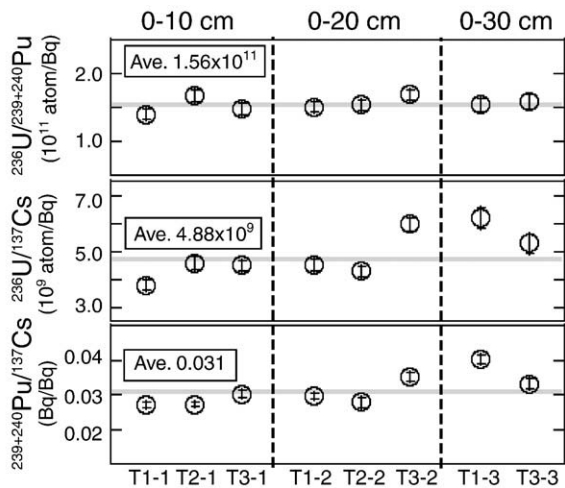
Fig. 2. Comparison of ratios among fallout nuclides, 239+240 Pu/ 137 Cs, 236 U/ 137 Cs and 236 U/ 239+240 Pu in the soil cores from Ishikawa pref. Japan. Gray lines show the average of ratios.
